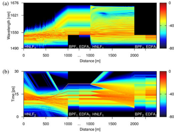
Fig. 5. Propagation of pulses in the cavity of Fig. 4(a). (a) In the frequency domain and (b) in the time domain. The propagation length of the BPFs and EDFAs are increased for readability.
